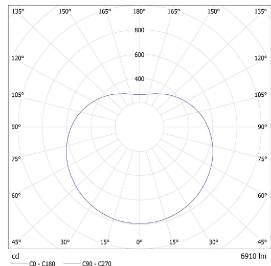
Lucis ZK.P2.600.X POLARIS ZK LED / LDC (Polar)
